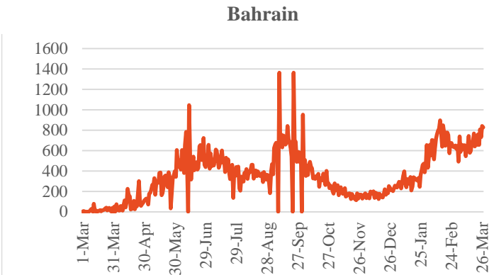
Figure 10: Comparative Analysis of the Distribution of COVID-19 New Cases in GCC Countries
